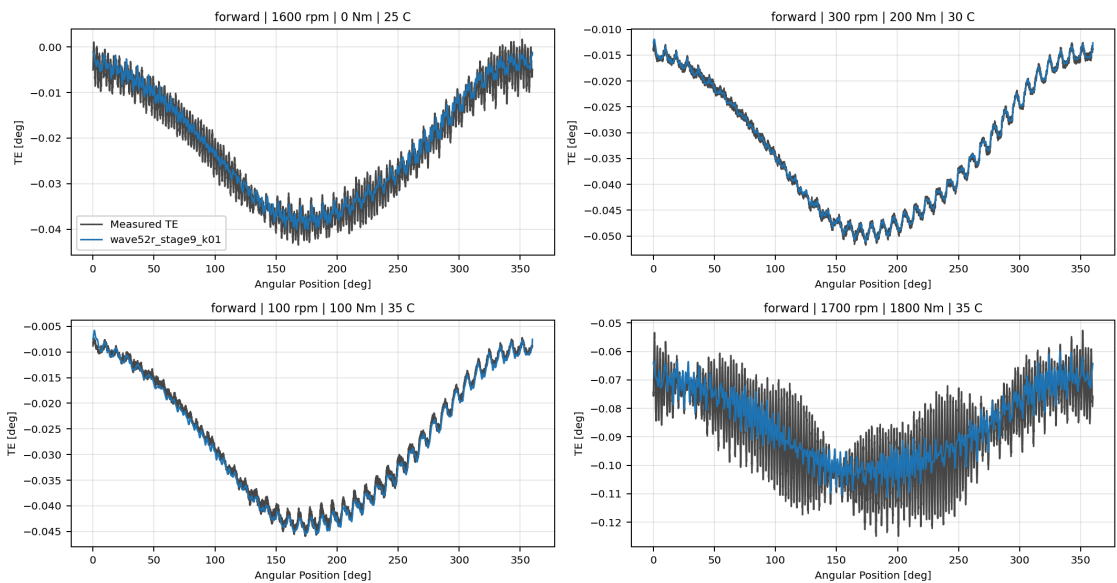
wave52r_stage9_k01 TE Curve Verification Pipeline collage
