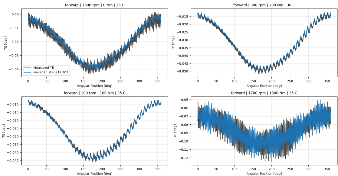
wave52r_stage12_f01 TE Curve Verification Pipeline collage
