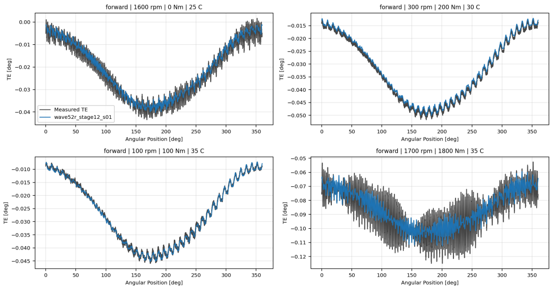
wave52r_stage12_s01 TE Curve Verification Pipeline collage
